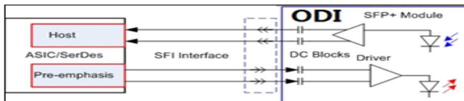
Figure1: Application in System
